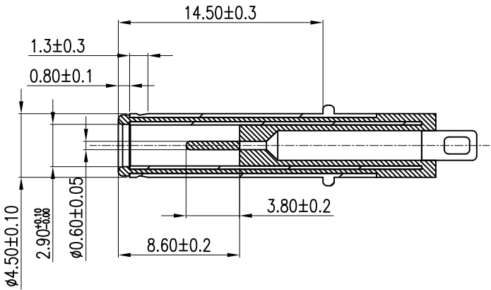
MATING PLUG (TOLERANCE:±0.05)
